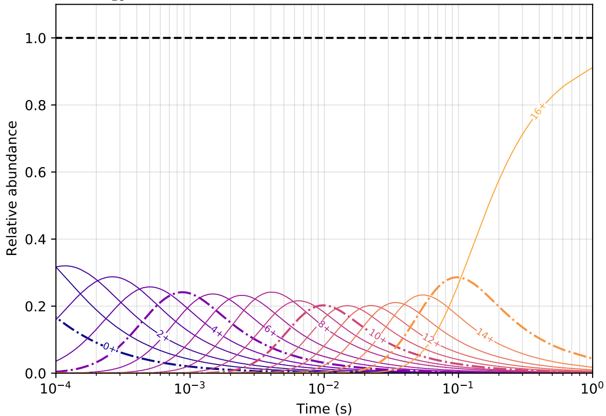
^{40}_{18}\text{Ar} charge states ( j = 200.0 \text{ A/cm}^2 , E_e = 2470.0 \text{ eV} )
