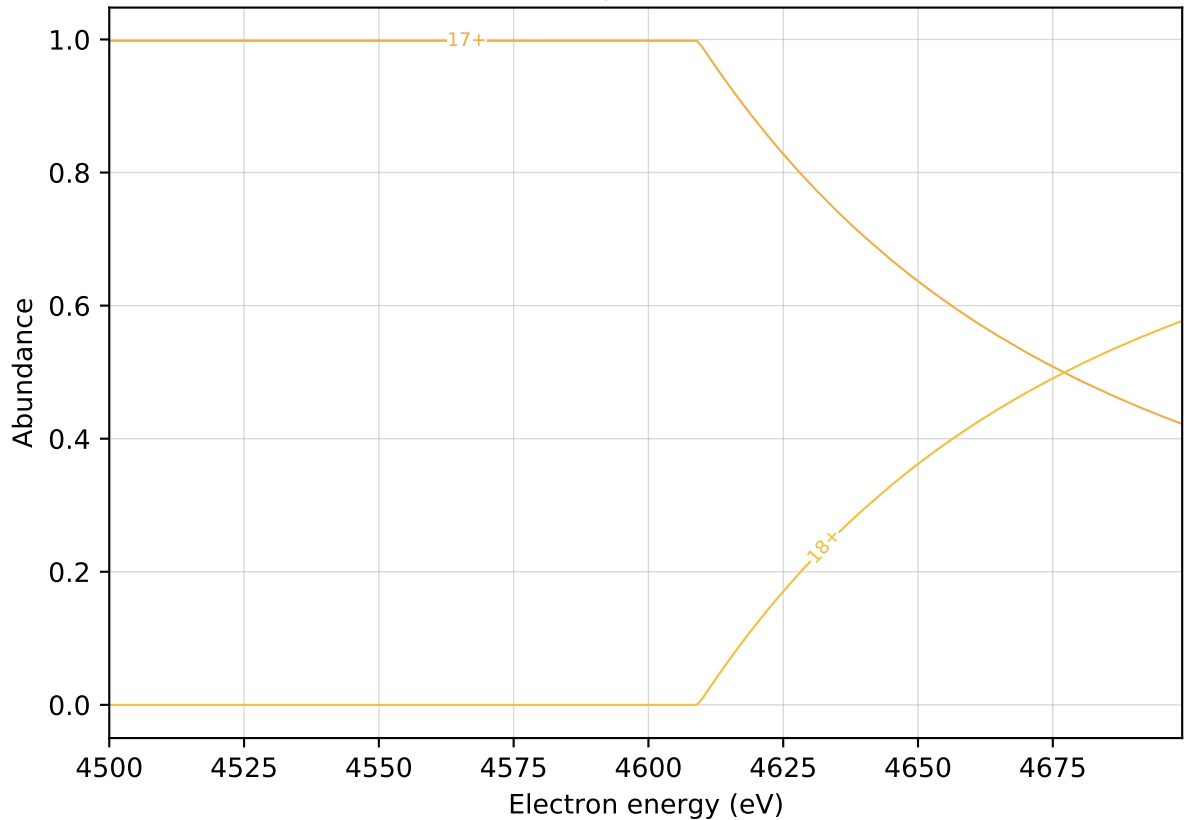
Abundance of ^{39}_{19}\text{K} at T = 20000.0 ms
