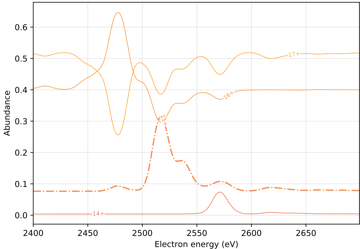
Abundance of ^{39}_{19}\text{K} at T = 100.0 ms
